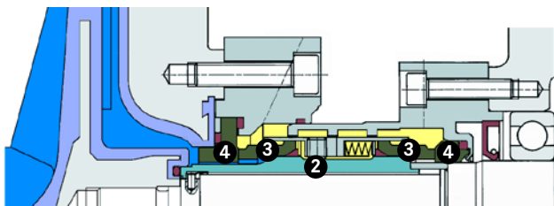
Back-to-back double mechanical seal
