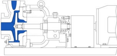
Bearing frame mounted ET with baseplate -20°C to +150°C
